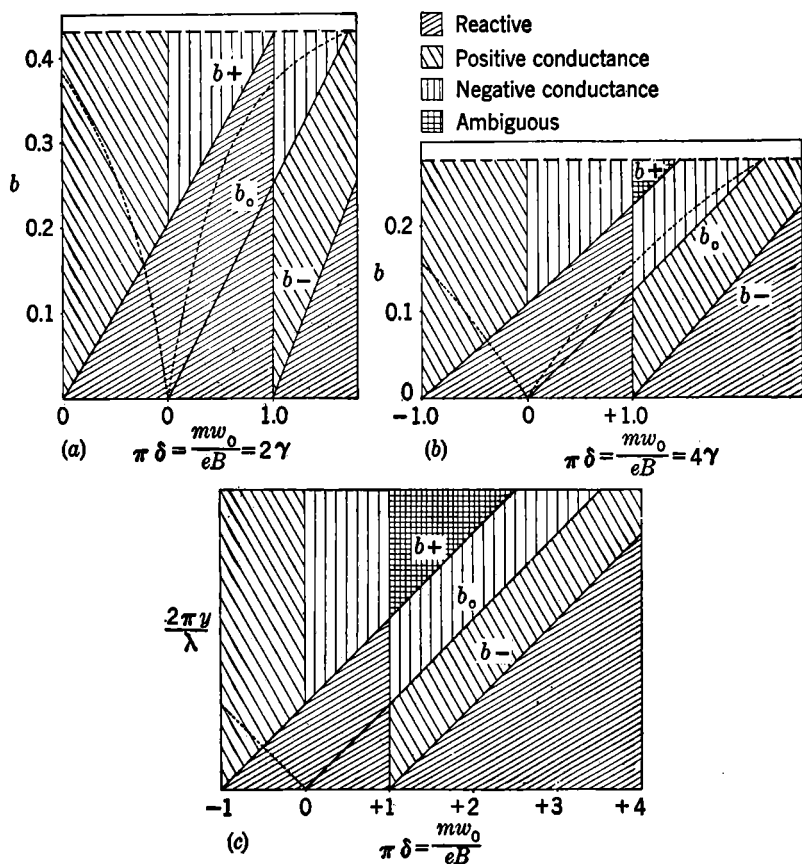
FIG. 6-13.—(a) Radii of the two singular streams and the stationary stream as a function of m\omega_0/eB for n = 4 . The function b = \frac{1}{2}(1 - r_{\text{cathode}}^2/r^2) is plotted. The broken line represents a typical value for the anode radius, and the dotted line indicates the cloud radius when the anode voltage is equal to the threshold voltage. (b) Same for n = 8 . (c) Location of the singular streams and stationary stream as a function of m\omega_0/eB for n = \infty . The variable 2\pi(y/\lambda_0) , where \lambda_0 is the wavelength of the field in the interaction space, is plotted. The cloud radius coincides with that of the stationary layer when the anode voltage is equal to the threshold voltage for each case.
